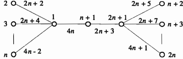
Fig. 4. Super (2n + 5, 3) -EAT labeling of S_{n,2,n}
